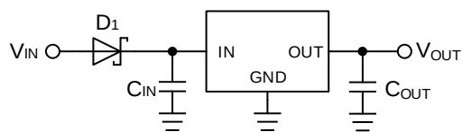
Figure 27. Protection against Reverse Polarity 1
