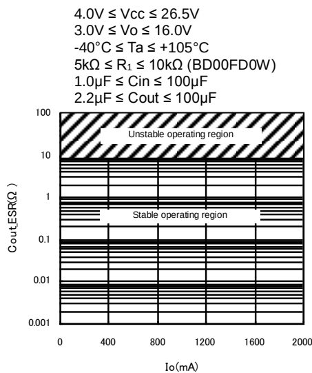
C_{out} ESR vs I_o 3.0\text{V} \leq V_o \leq 16.0\text{V}
