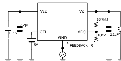
Measurement setup for Figure 16.
