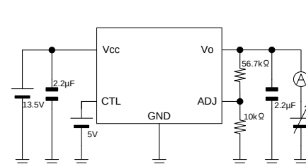
Measurement setup for Figure 11,12.
