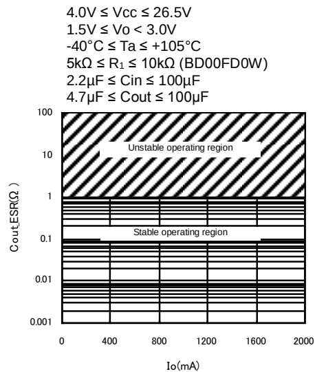
C_{out} ESR vs I_o 1.5\text{V} \leq V_o < 3.0\text{V}
