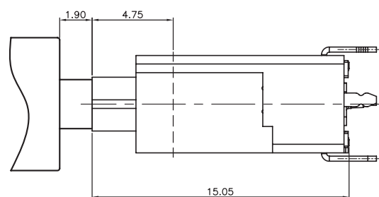
MATING CONDITION
