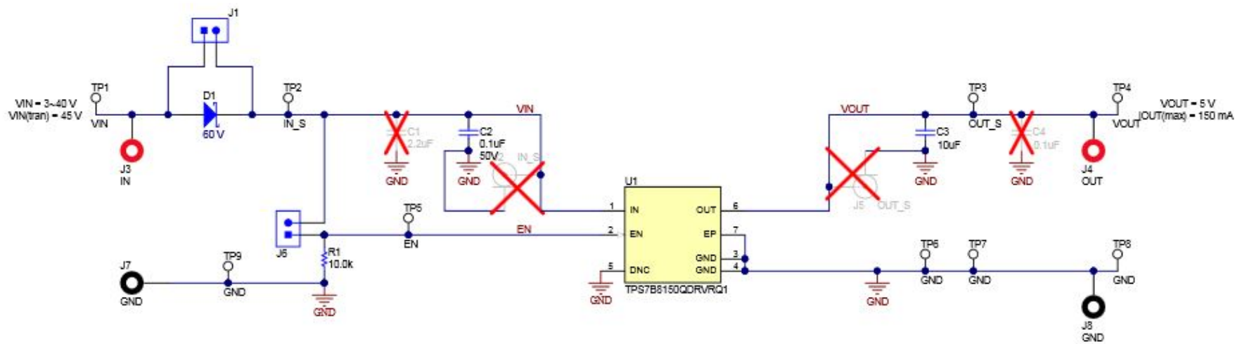
Figure 4. TPS7B81EVM-025 Schematic
