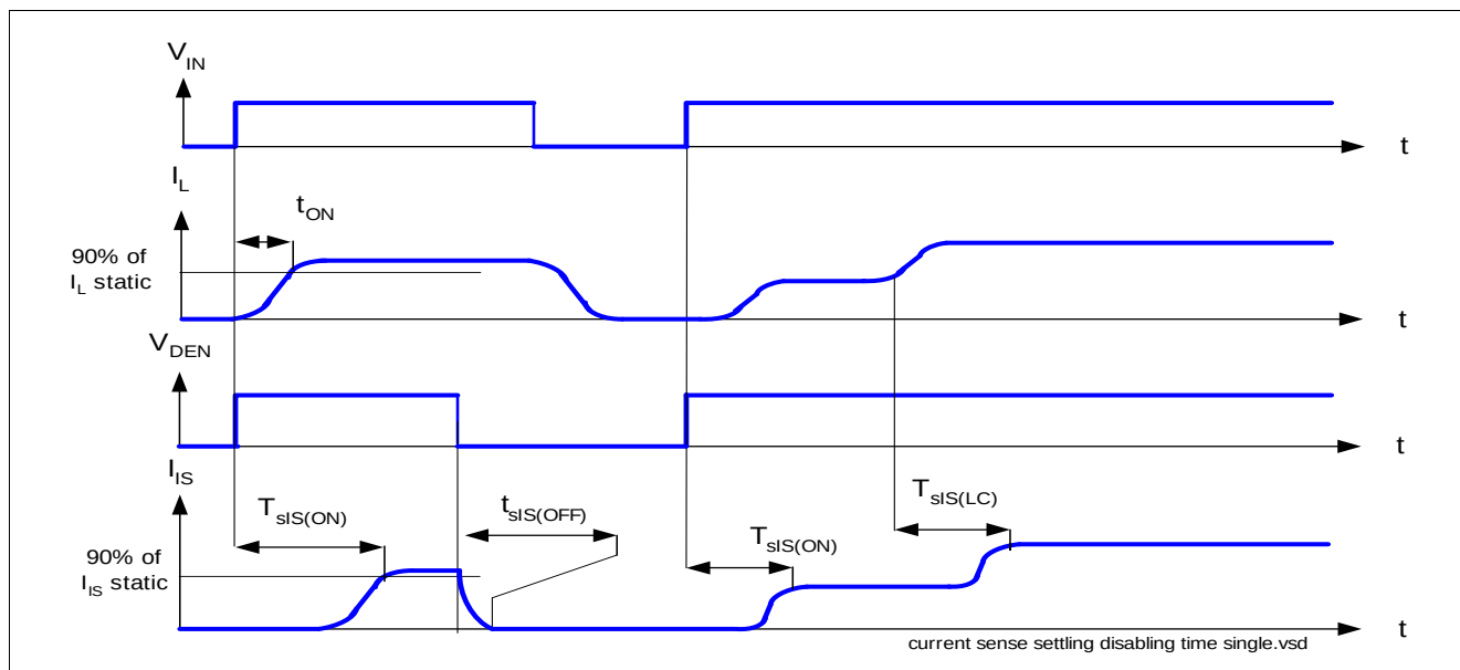
Figure 23 SENSE Settling / Disabling Timing
