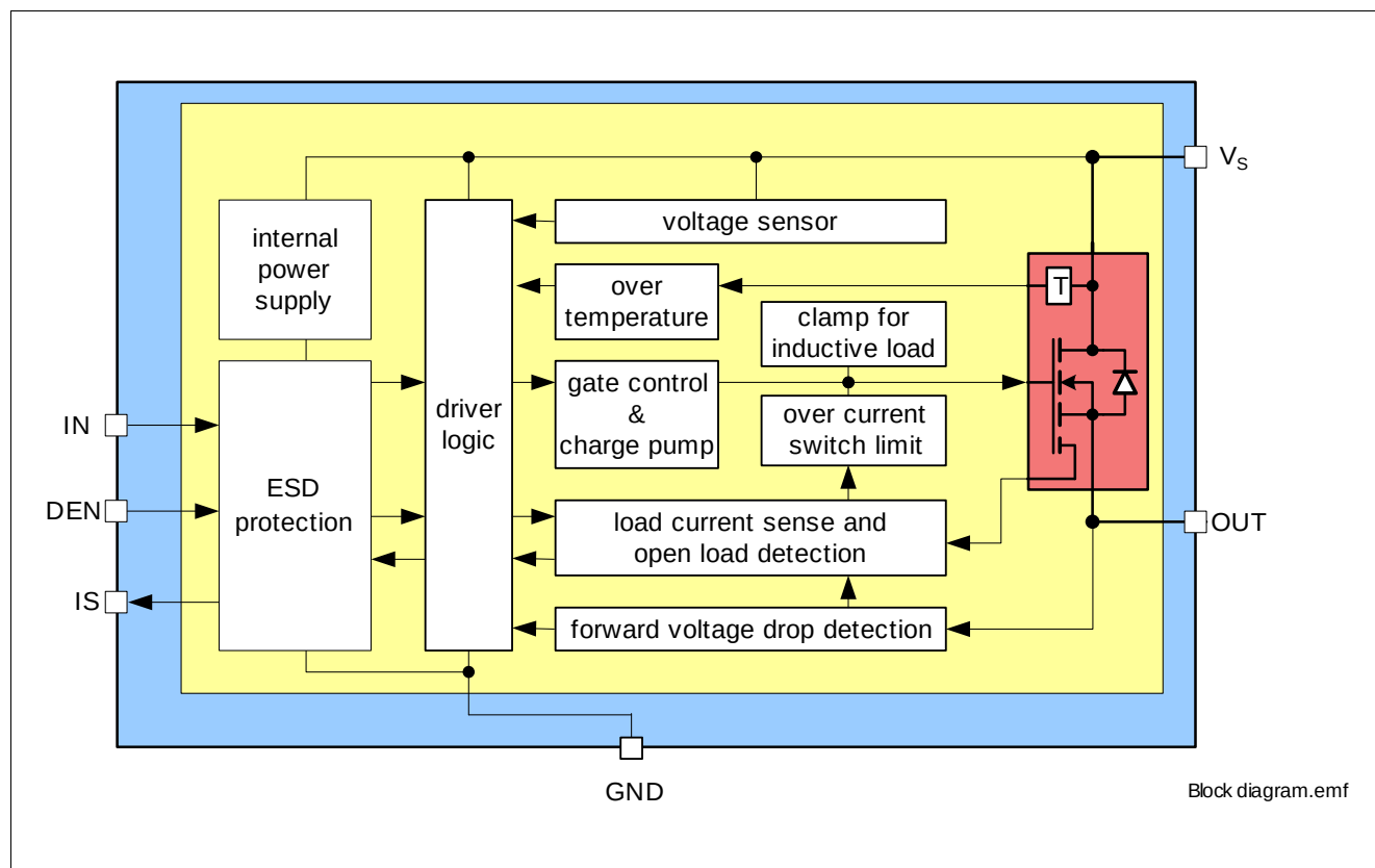
Figure 1 Block Diagram for the BTS5030-1EJA
