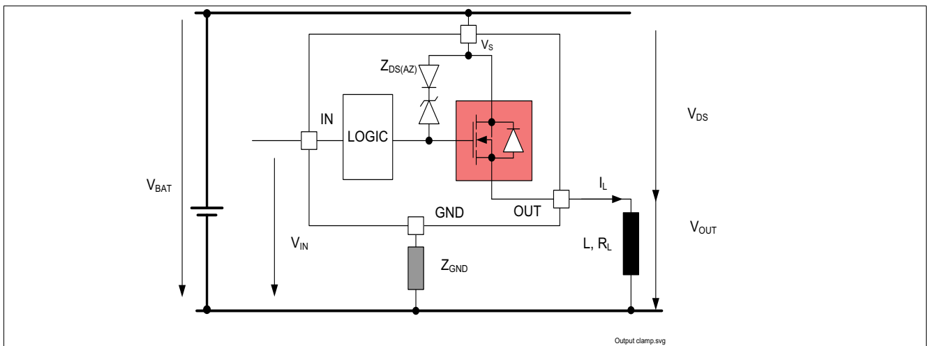
Figure 10 Output Clamp
