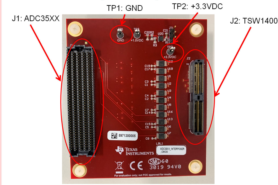
Figure 2-2. CMOS FPGA Interposer Card
