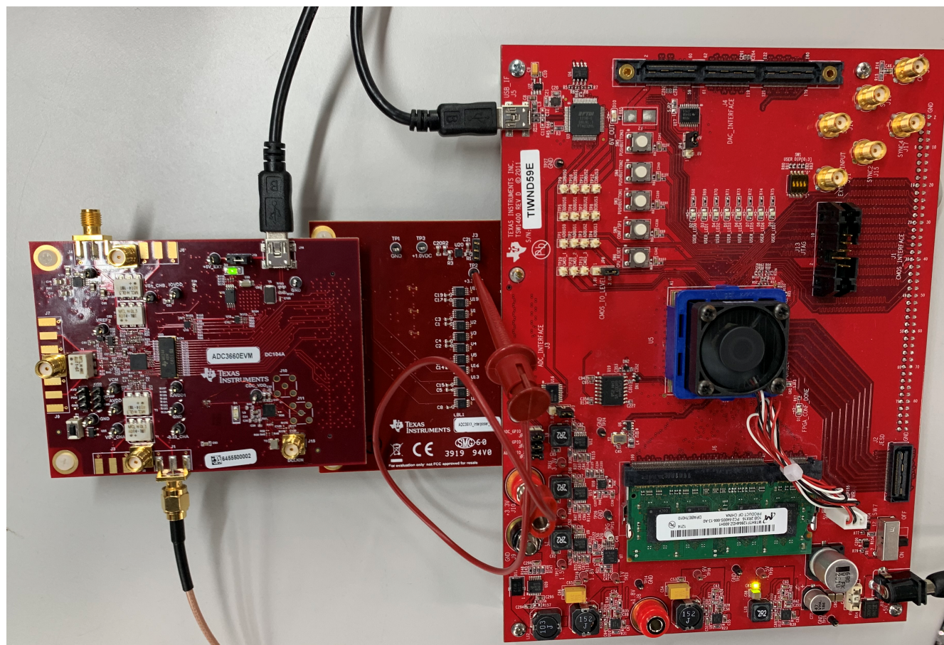
Figure 3-1. ADC360EVM Full Setup
