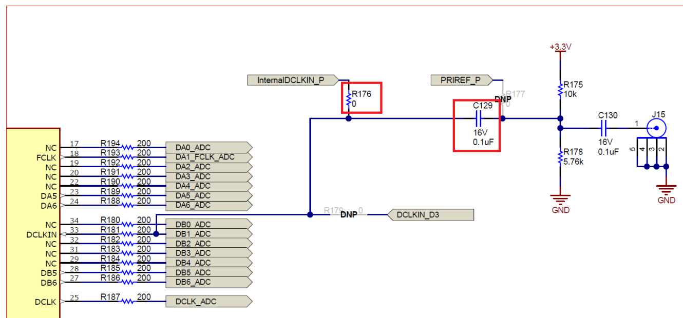
Figure 5-2. ADC364xEVM Schematic Snippet: DCLKIN
