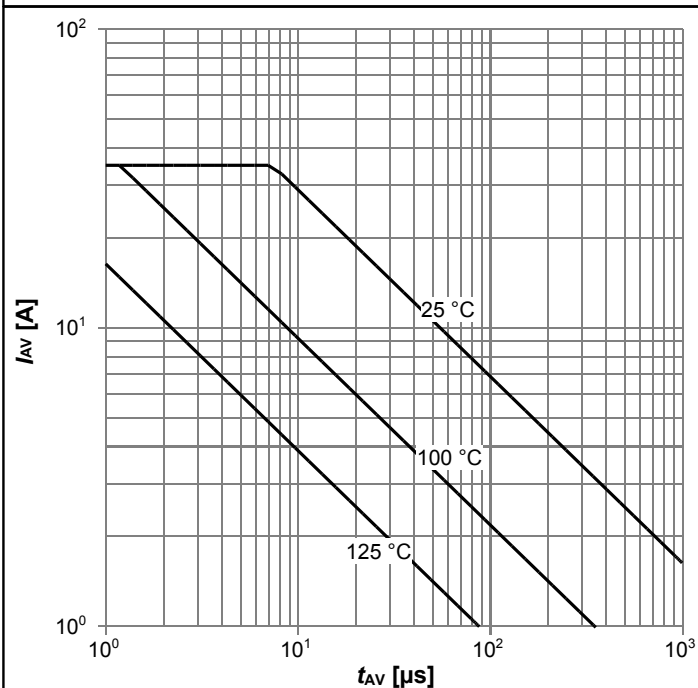
Diagram 13: Avalanche characteristics
