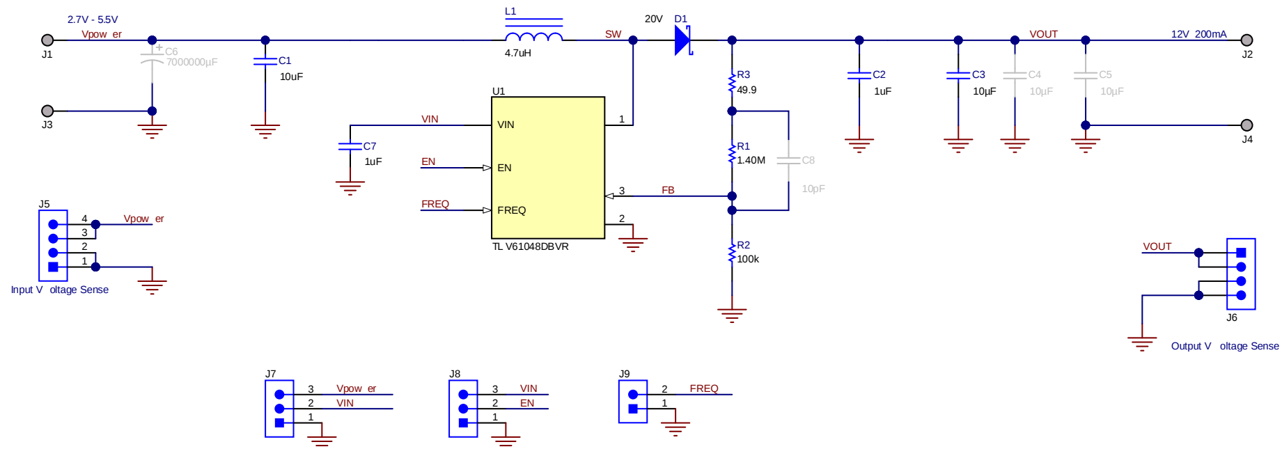
Figure 1. TLV61048EVM-042 Schematic
