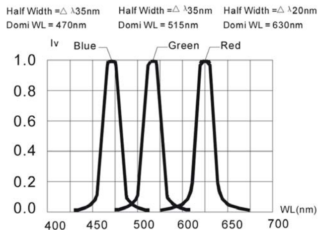
Fig.4 Relative Luminous Intensity vs. Wavelength
