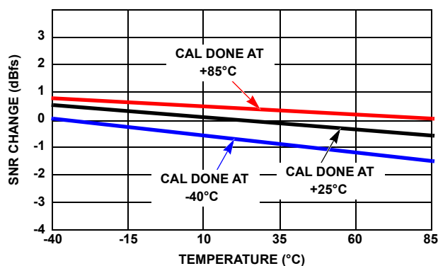
FIGURE 28. SNR PERFORMANCE vs TEMPERATURE AFTER +25^{\circ}\text{C} CALIBRATION
