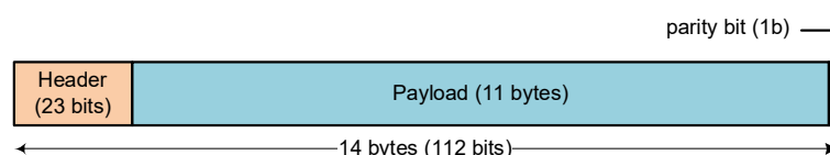
Figure 36. PWM Frame
