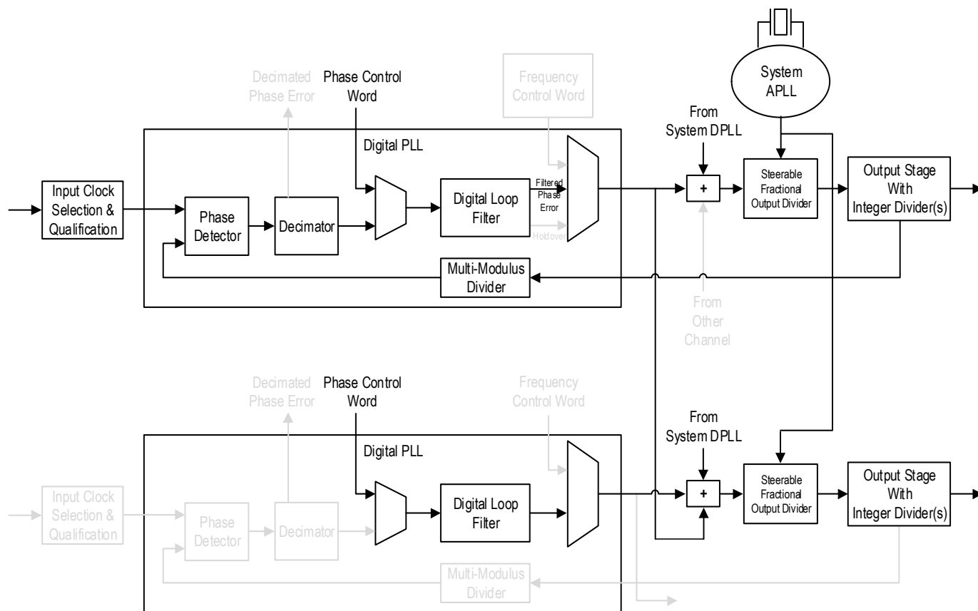
Figure 31. Combo Mode
