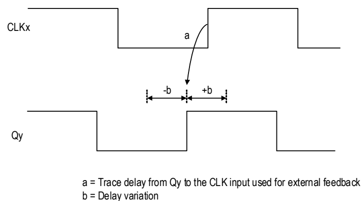
Figure 43. Input-Output Delay with External Feedback
