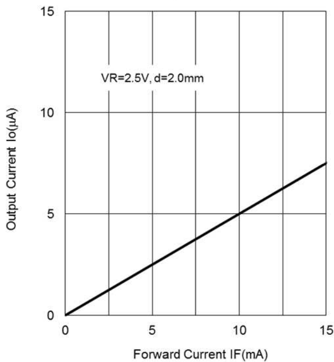
Output Current vs. Forward Current ( T_a=25^\circ\text{C} )
