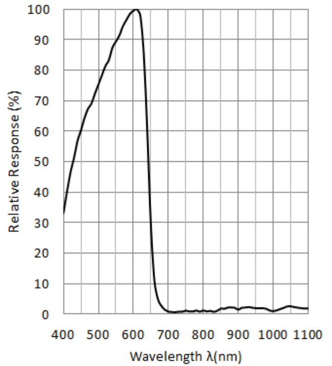
Spectral Response ( T_a=25^\circ\text{C} ) Detector PD
