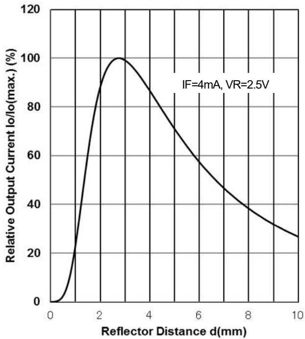
Output current vs. Distance (Ta=25°C)
