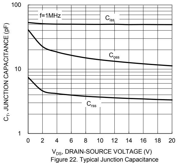
Figure 22. Typical Junction Capacitance
