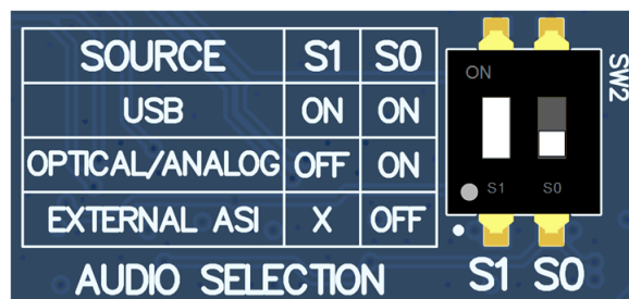
Figure 2-4. AC-MB External Audio Setting
