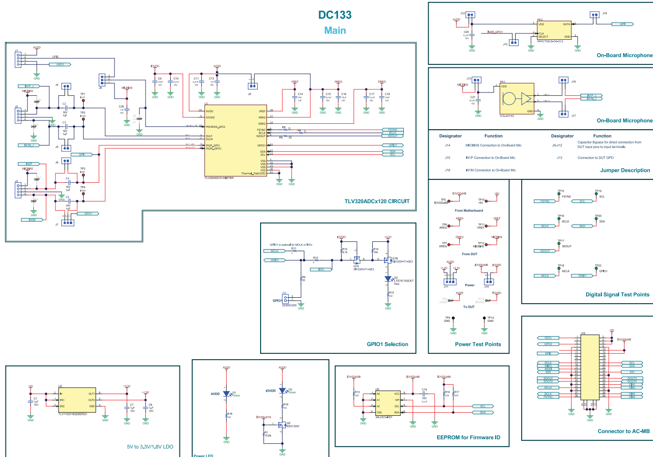
Figure 7-1. ADCx120EVM-PDK Schematics
