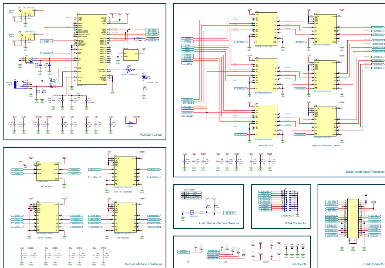
Figure 7-2. AC-MB Schematics
