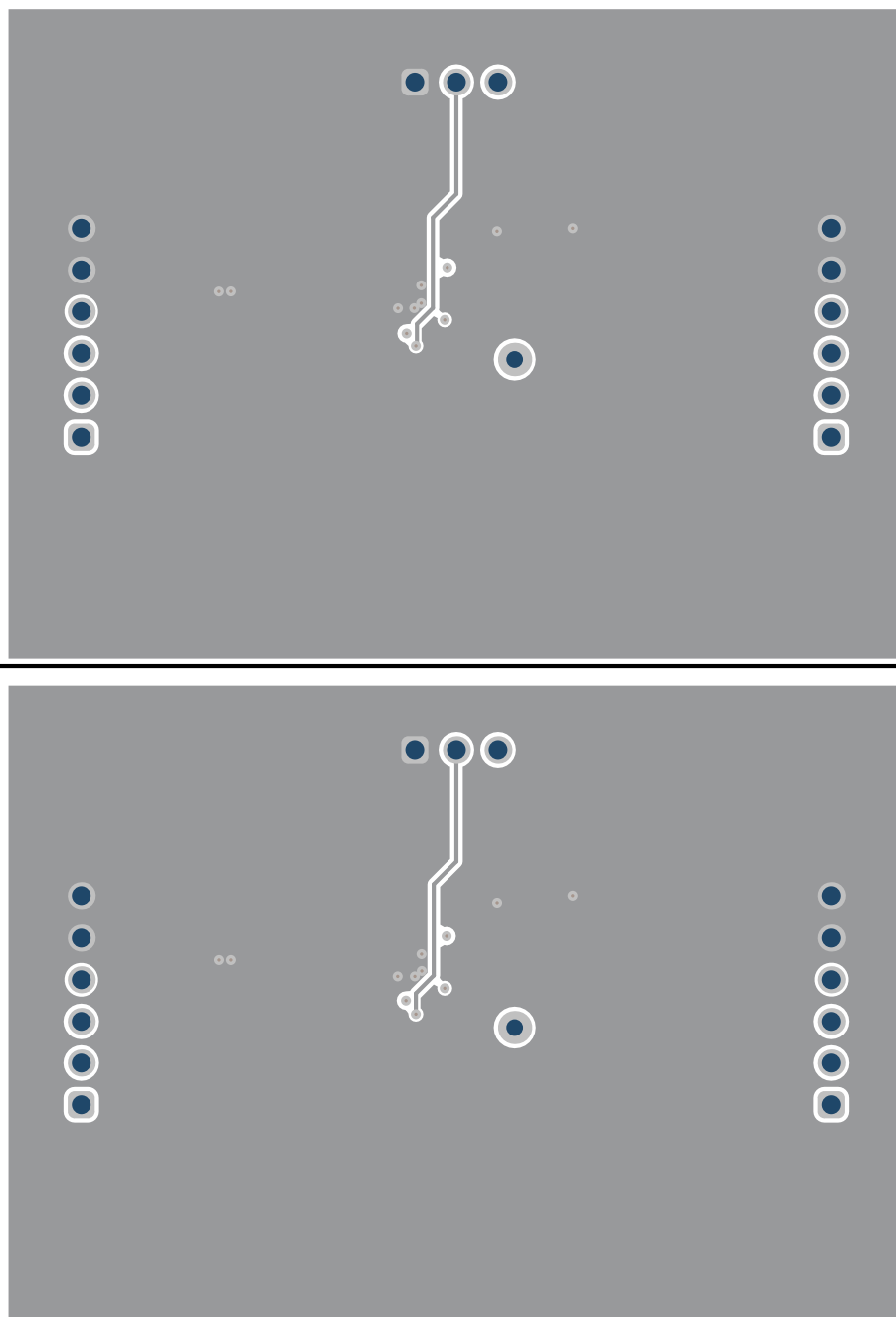
Figure 7. Internal Layer 2
