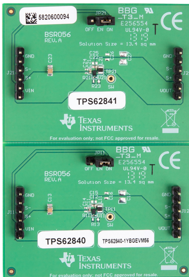
Figure 10. TPS62840-1YBGEVM56 Overhead View
