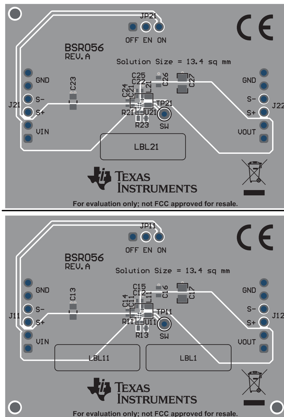
Figure 4. Top Assembly
