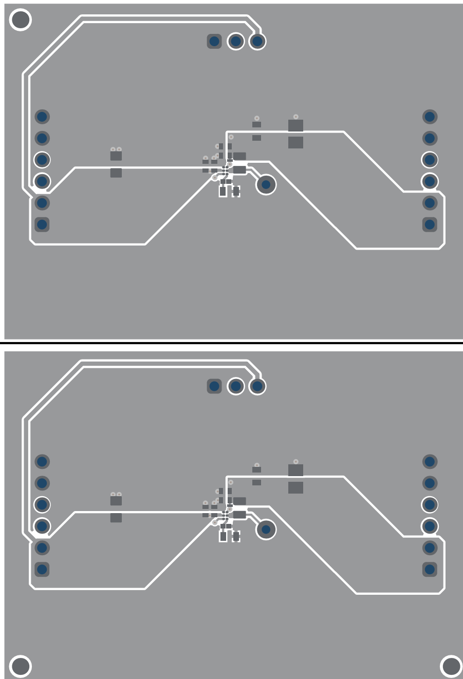
Figure 5. Top Layer
