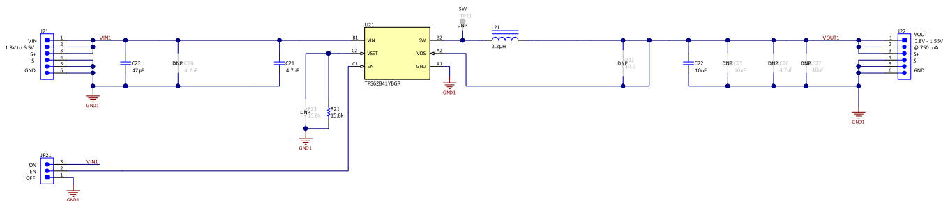
Figure 12. TPS62841 Schematic
