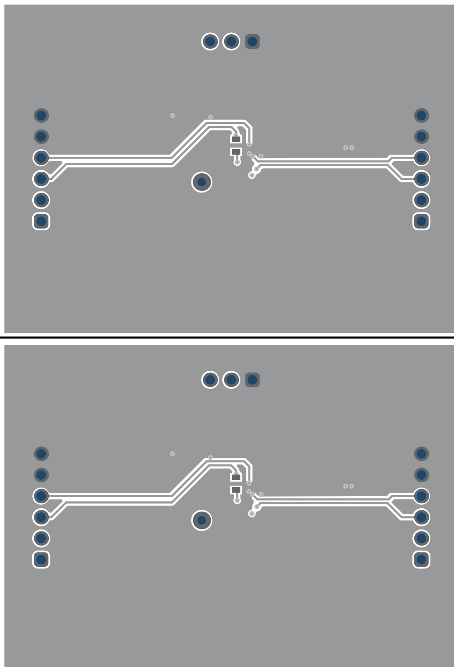
Figure 8. Bottom Layer
