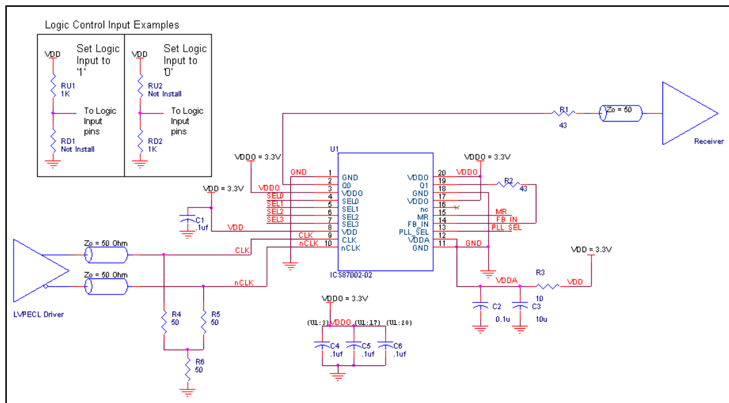
Figure 4. 87002-02 Schematic Example
