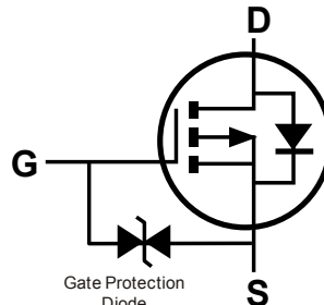
Internal Schematic
