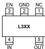
MIC3490 5-Pin SOT23 (Top View)
