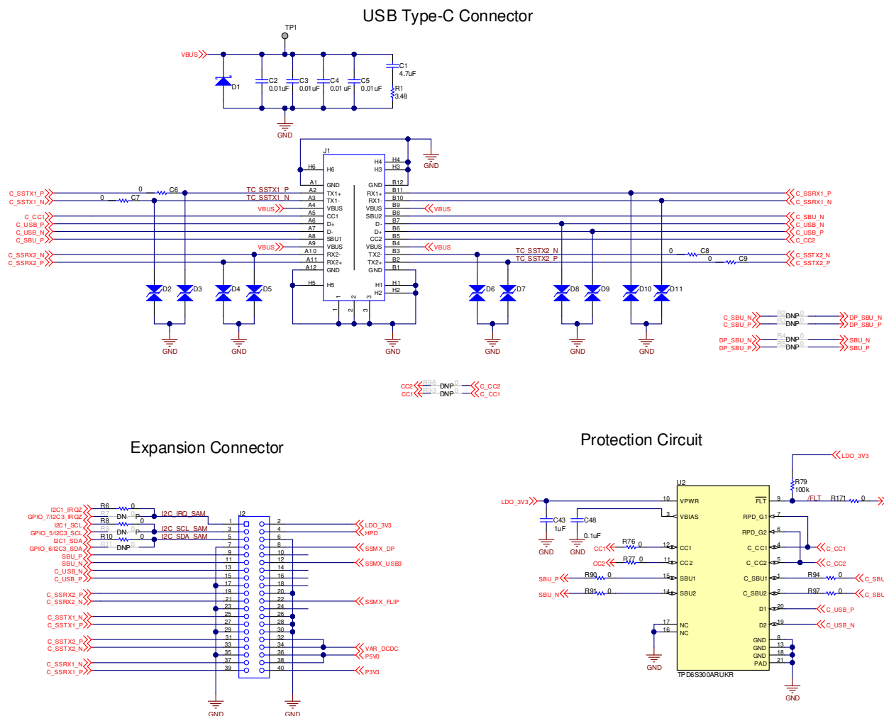
Figure 4. USB Type-C™ and External Module Connectors
