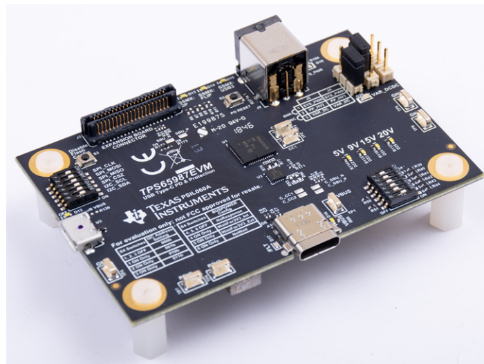
Figure 1. TPS65987EVM Board
