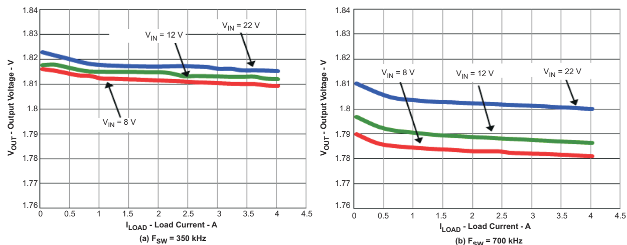
Figure 7-4. Output Voltage vs Load ( V_{IN} = 8\text{ V} – 22\text{ V} , V_{OUT2} = 1.8\text{ V} , I_{OUT2} = 0\text{ A} – 4\text{ A} )
