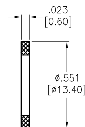
O-RING
