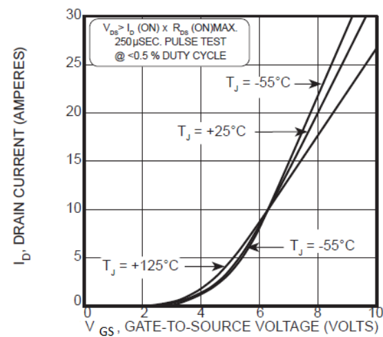
Figure 1-3. Transfer Characteristics
