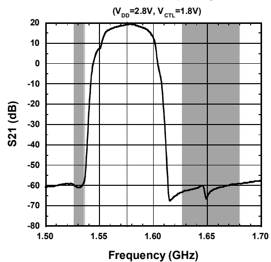
S21 vs. Frequency
