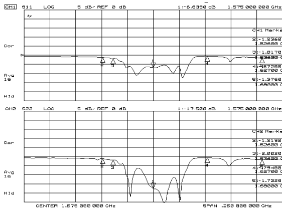
S11, S22
