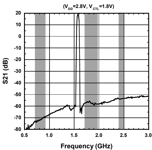
S21 vs. Frequency
