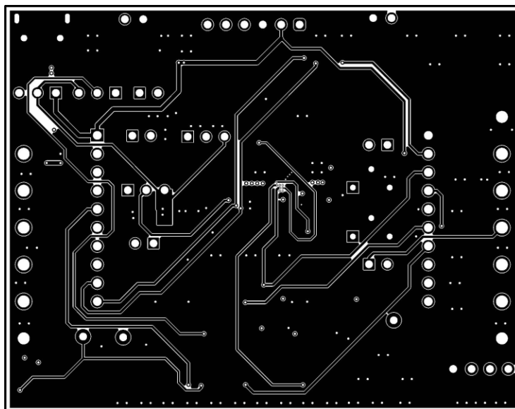
Figure 8. Bottom Layer
