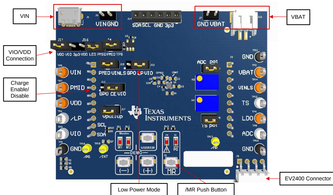
Figure 1. BQ2515xEVM Connections
