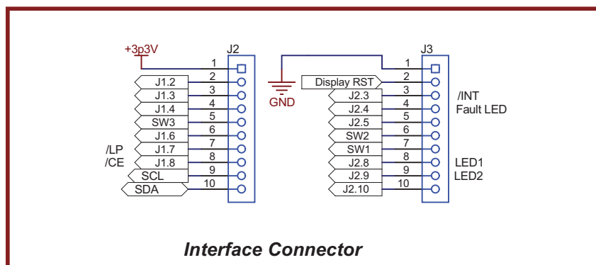
Figure 16. BQ2515xEVM Interface Connector
