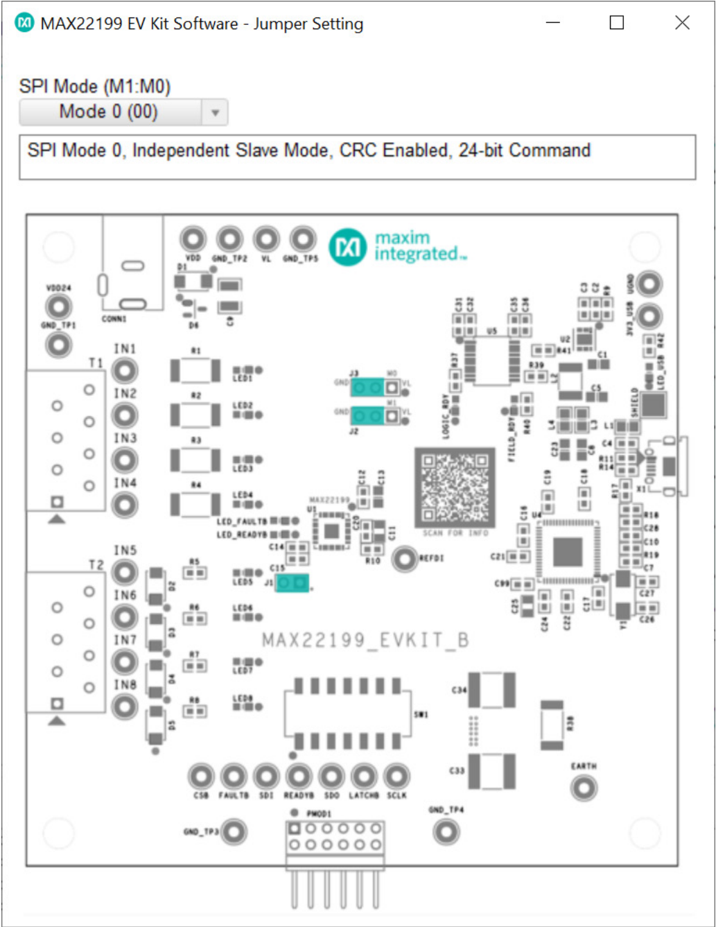
Figure 5. MAX22199 EV Kit Software—Jumper Setting Diagram
