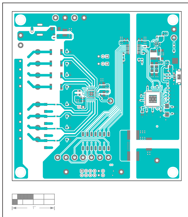
MAX22199 EV Kit PCB Layout—Top
