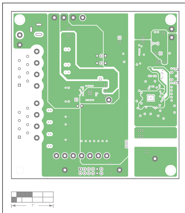
MAX22199 EV Kit PCB Layout—Internal 3
