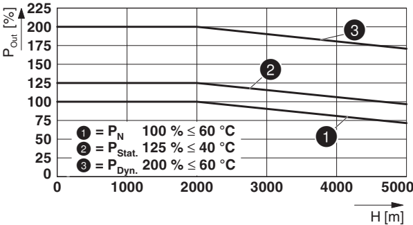
Figure 47 Output power depending on the installation height
