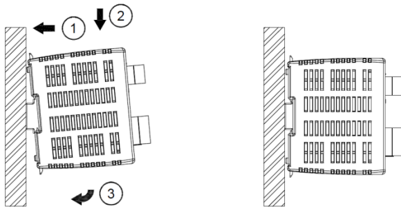
Fig. 2.1 Mounting
