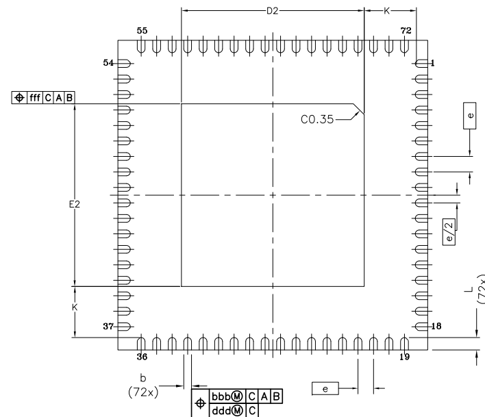
BOTTOM VIEW
