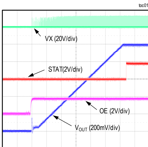
STARTUP RESPONSE
