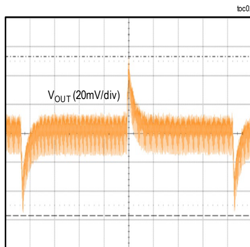
TRANSIENT RESPONSE
