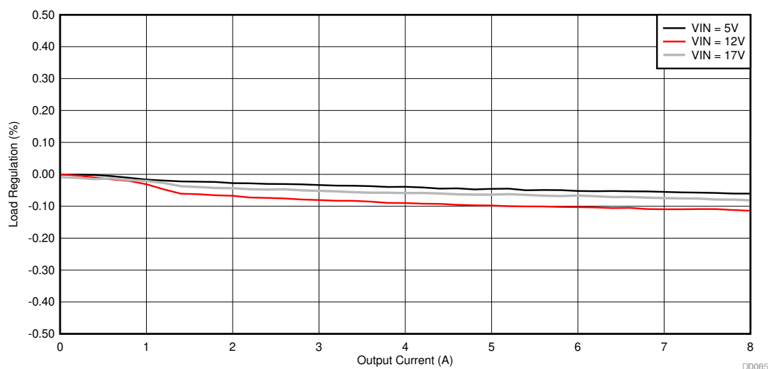
Figure 2-4. TPS54824EVM-779 Load Regulation
