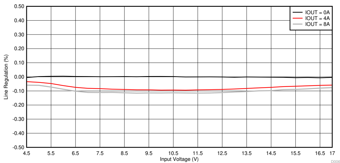
Figure 2-5. TPS54824EVM-779 Line Regulation
