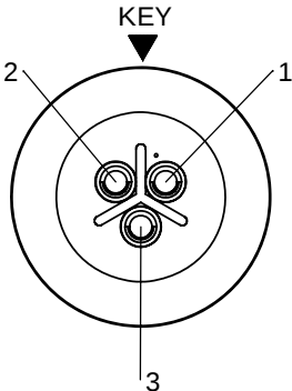
WIRING END W7382-3PG-P-300
