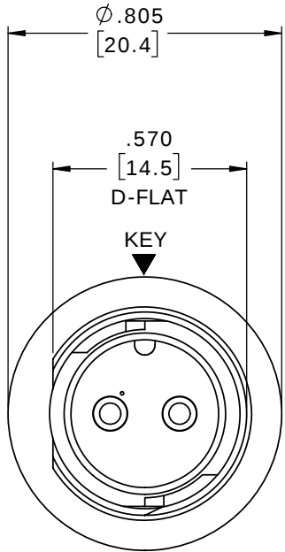
MATING FACE W7382-2PG-P-300 SHOWN
