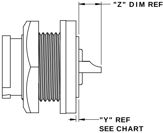
ASSEMBLED VIEW W7382-2PG-P-300 SHOWN
