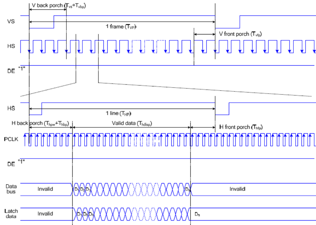
Timing chart of RGB interface HV mod
