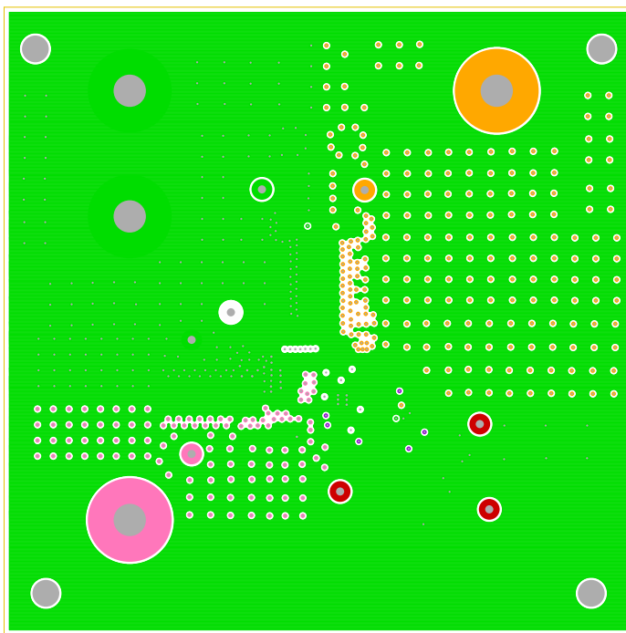
Figure 9. Inner Layer 2
