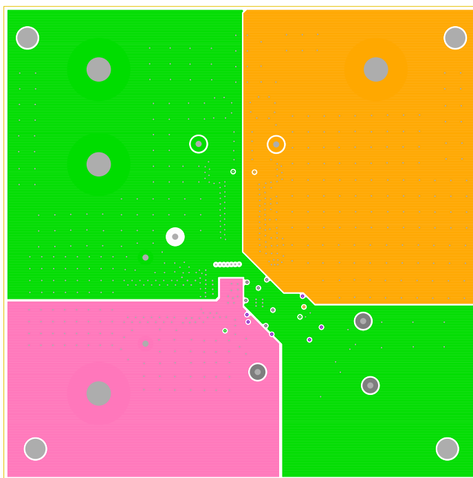
Figure 11. Inner Layer 4
