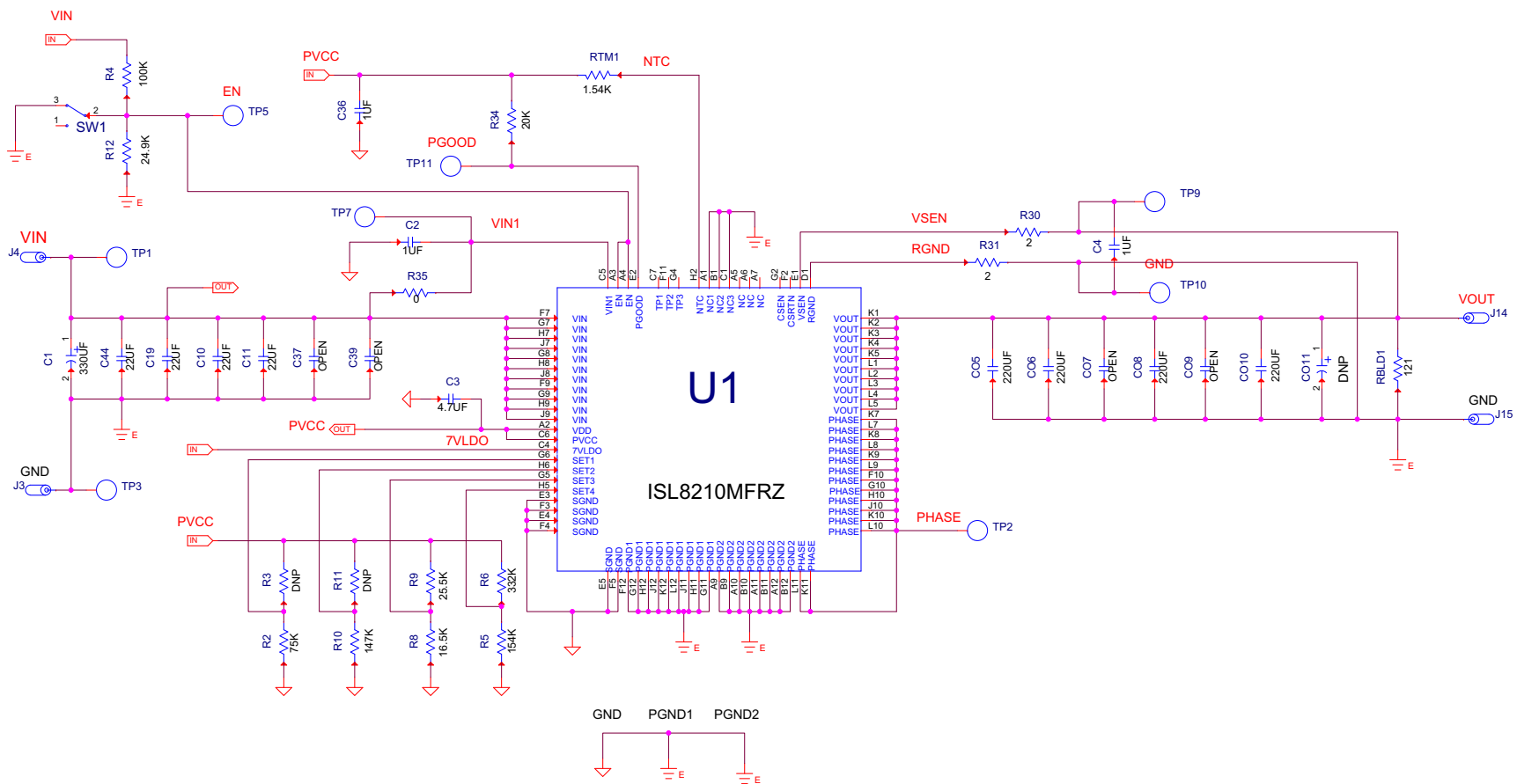
Figure 6. Schematic
