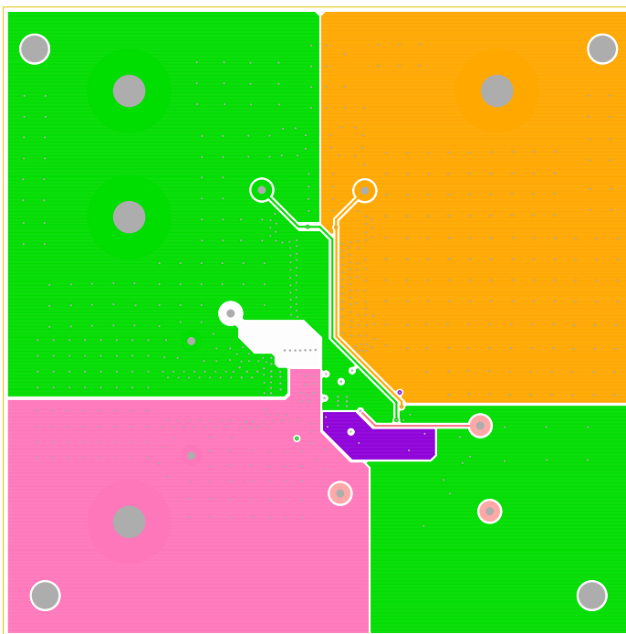
Figure 10. Inner Layer 3
