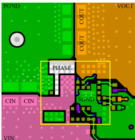
Figure 2. Layout Example - Top Layer
