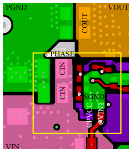
Figure 3. Layout Example - Bottom Layer
