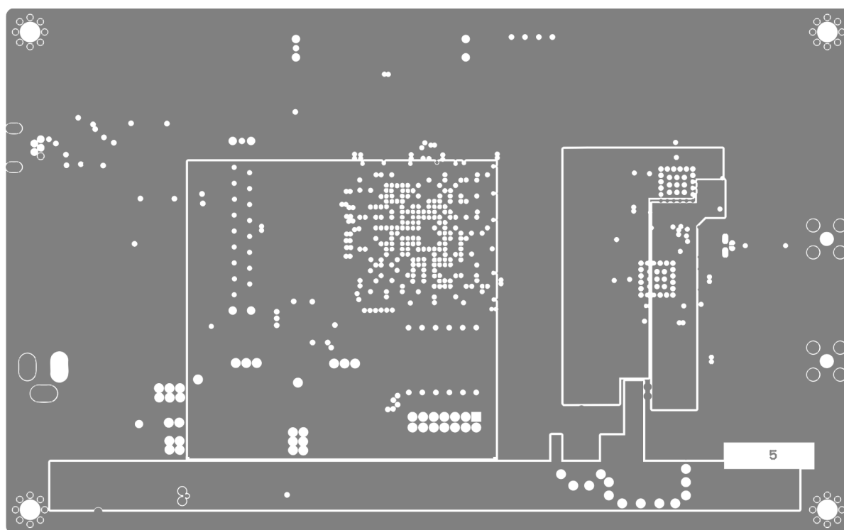
Figure 10. Layer 5
