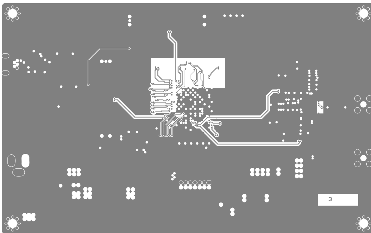
Figure 8. Layer 3
