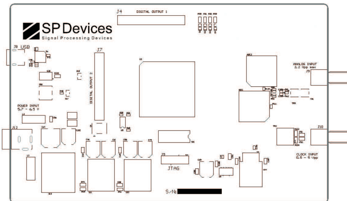
Figure 1. Board Layout
