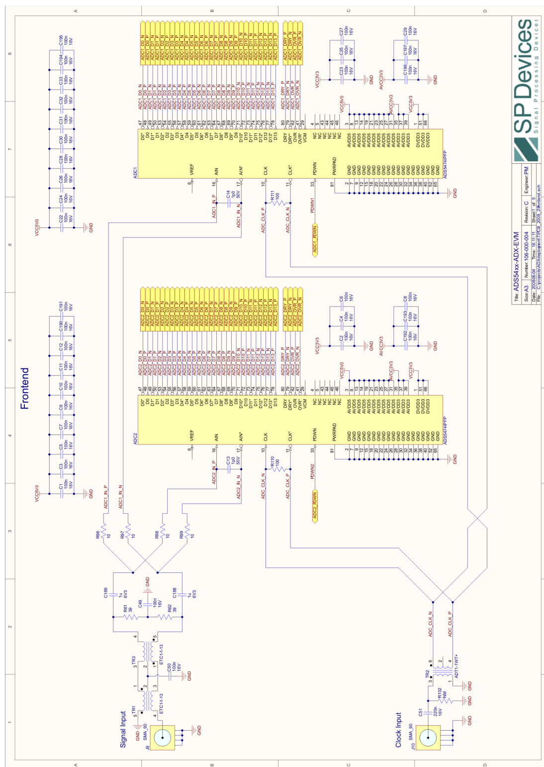
Figure 14. Front End Schematic
