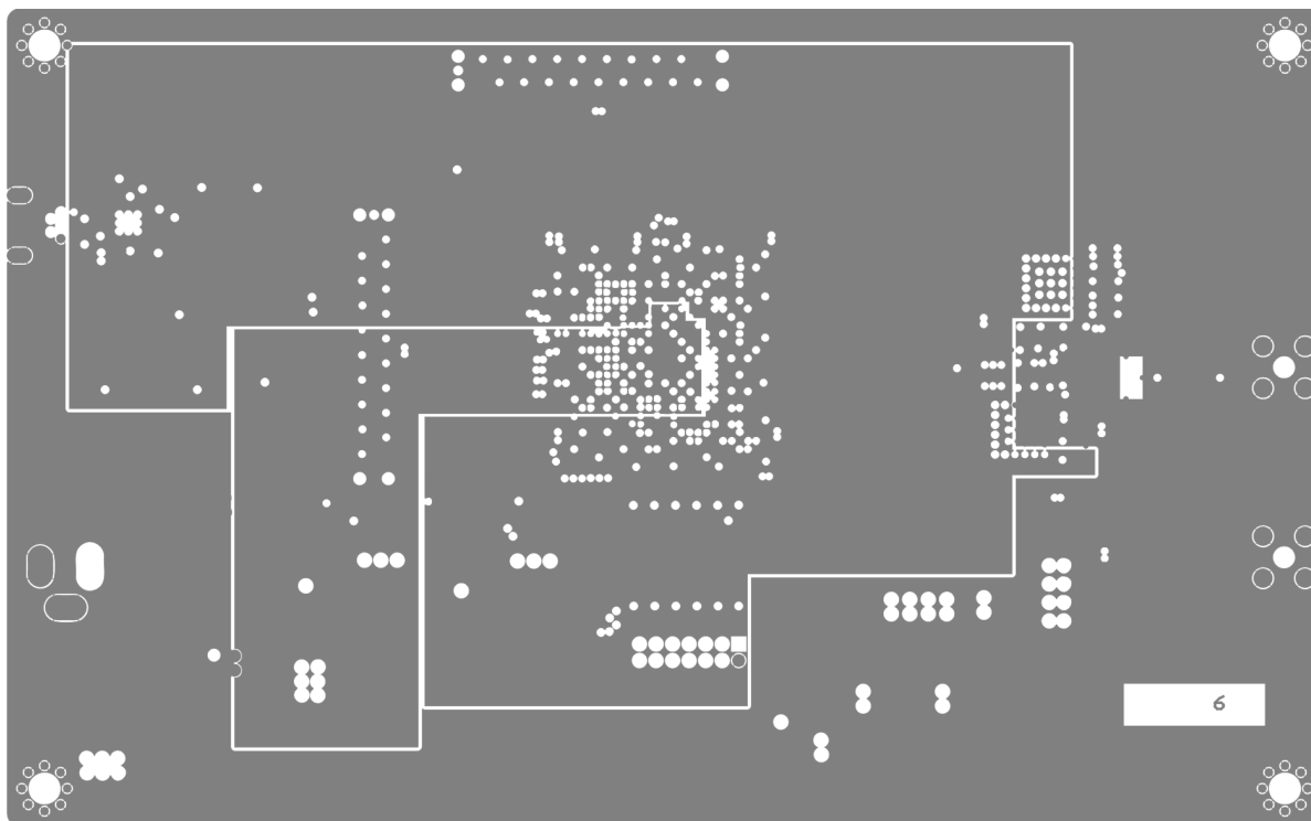
Figure 11. Layer 6
