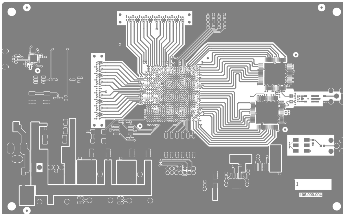
Figure 6. Layer 1
