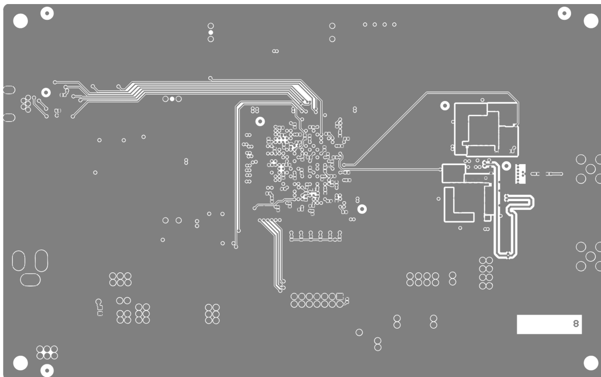
Figure 13. Layer 8
