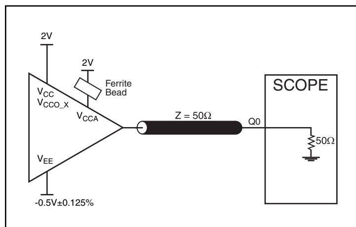
2.5V/2.5V QAx_CMOS Output Load Test Circuit
