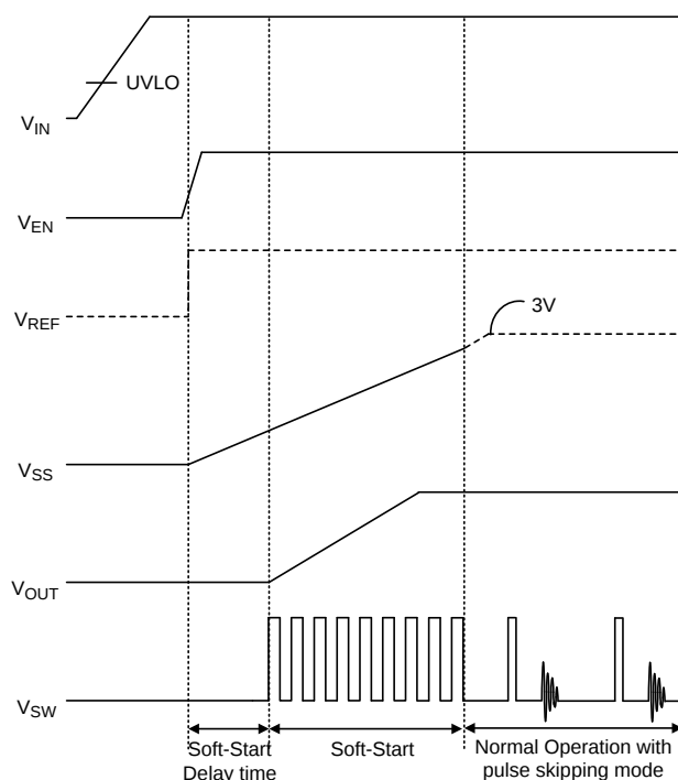
Figure 2. Power-Up Sequence Controlled by the EN Pin
