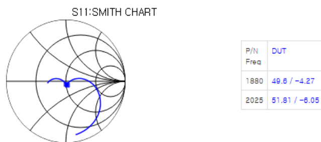
Smith Chart (Input Port)
