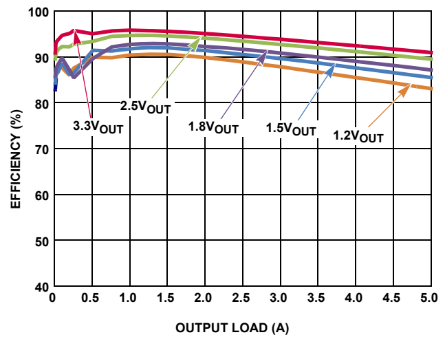
FIGURE 8. EFFICIENCY vs LOAD ( 5V_{IN} ; \text{SYNC} = \text{GND} )
