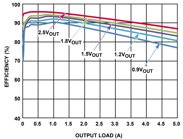
FIGURE 6. EFFICIENCY vs LOAD ( 3.3V_{IN} ; \text{SYNC} = \text{GND} )
