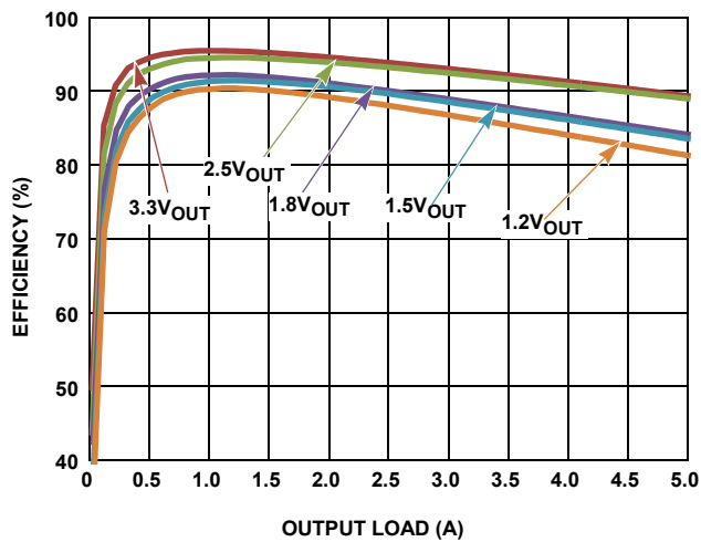
FIGURE 7. EFFICIENCY vs LOAD ( 5V_{IN} ; \text{SYNC} = V_{DD} )
