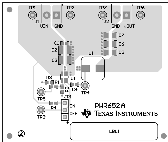
Figure 5-1. Top Assembly
