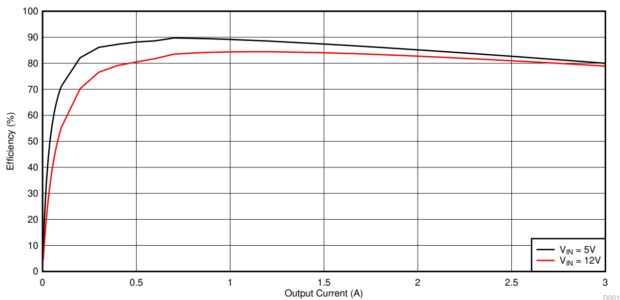
Figure 4-1. TPS563209EVM-652 Efficiency
