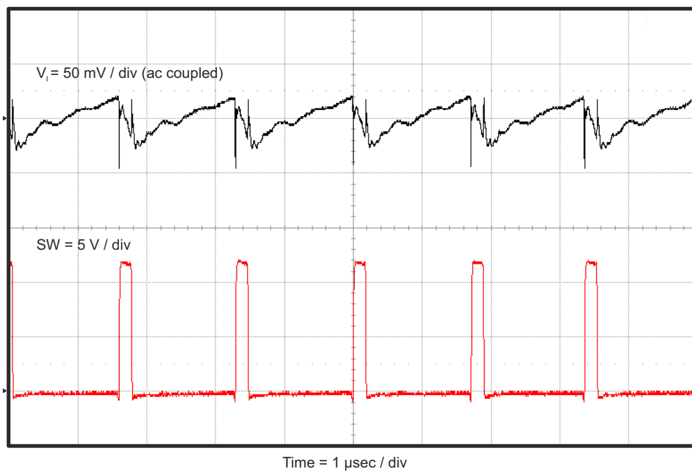
Figure 4-9. TPS563209EVM-652 Input Voltage Ripple, I_{\text{OUT}} = 3 \text{ A}
