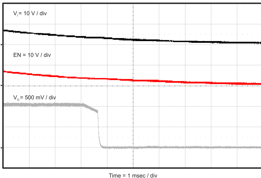
Figure 4-12. TPS563209EVM-652 Shut-Down Relative to V_{IN}
