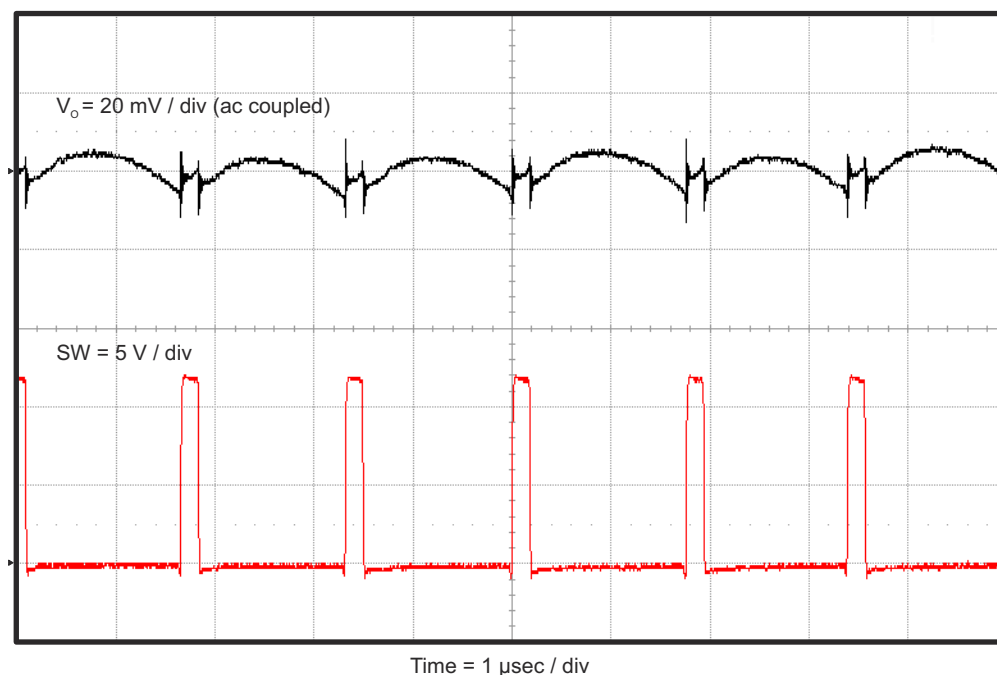
Figure 4-7. TPS563209EVM-652 Output Voltage Ripple, I_{\text{OUT}} = 3 \text{ A}
