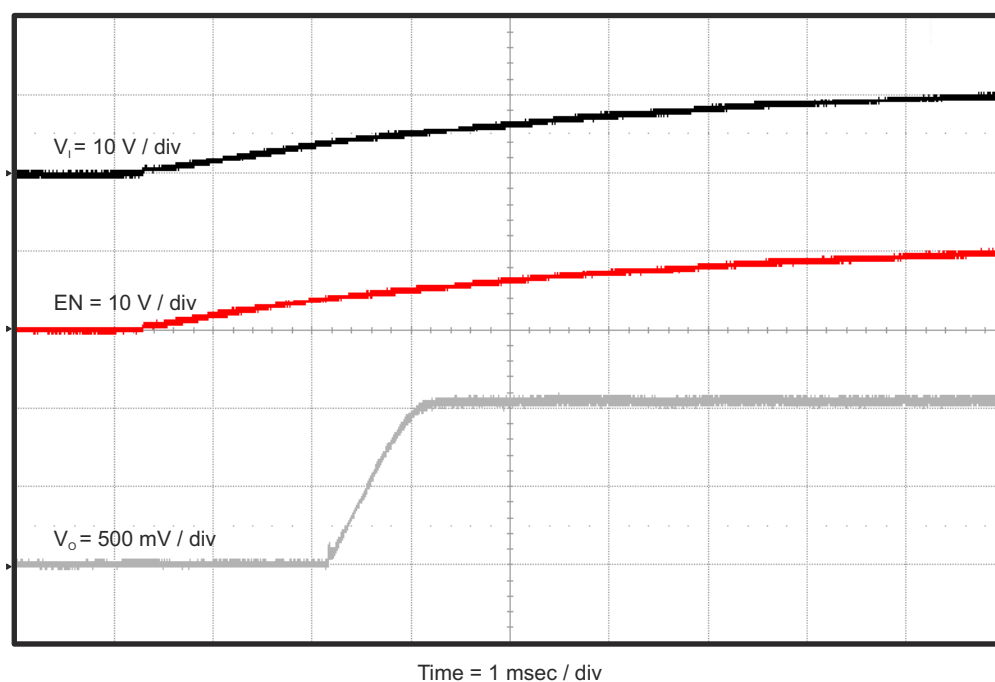
Figure 4-10. TPS563209EVM-652 Start-Up Relative to V_{IN}
