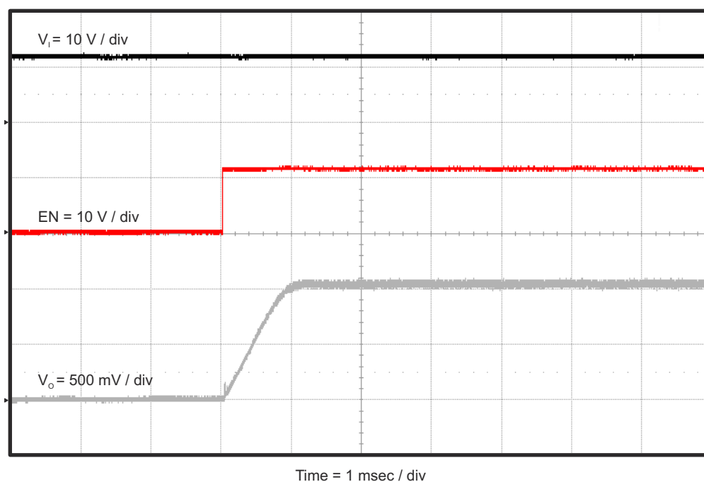
Figure 4-11. TPS563209EVM-652 Start-Up Relative to EN
