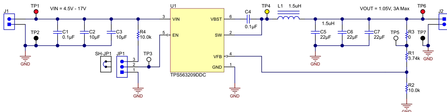
Figure 6-1. TPS563209EVM-652 Schematic Diagram
