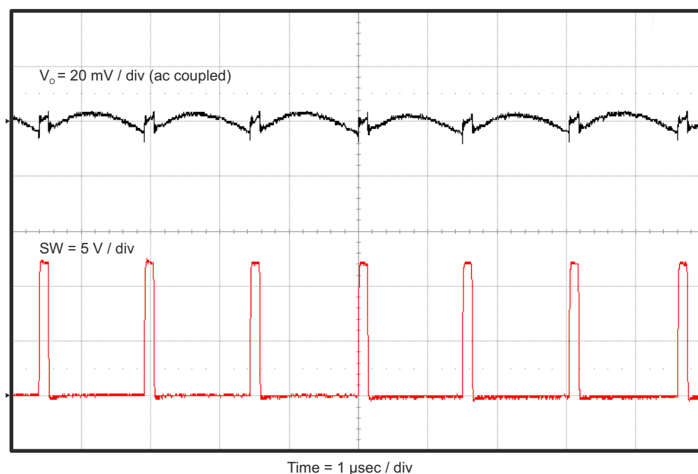
Figure 4-8. TPS563209EVM-652 Output Voltage Ripple, I_{\text{OUT}} = 0 \text{ mA}
