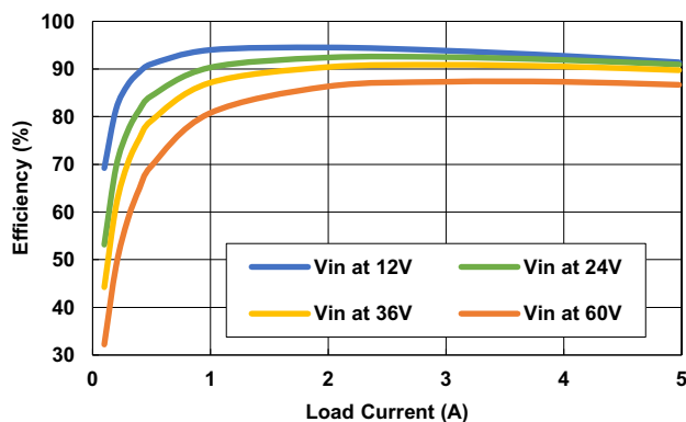
Figure 15. Efficiency vs Load Current ( V_{OUT} = 5V , L = 4.7\mu H , C_{OUT} = 70\mu F )
