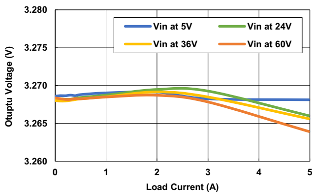
Figure 18. Load Regulation
