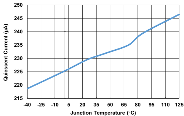
Figure 4. PVIN Quiescent Current vs Junction Temperature
