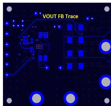
Figure 65. Bottom Layer
