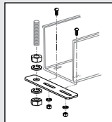
FTRBN12 – New Threaded Rod Bracket (page J.48)
