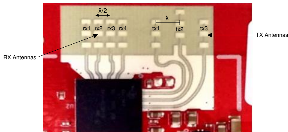
Figure 10. PCB Antenna
