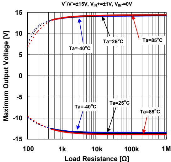
Maximum Output Voltage vs. Load Resistance
