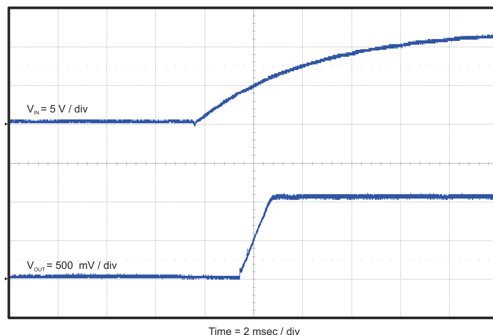
Figure 4-8. TPS54429EEVM-608 Start-Up
