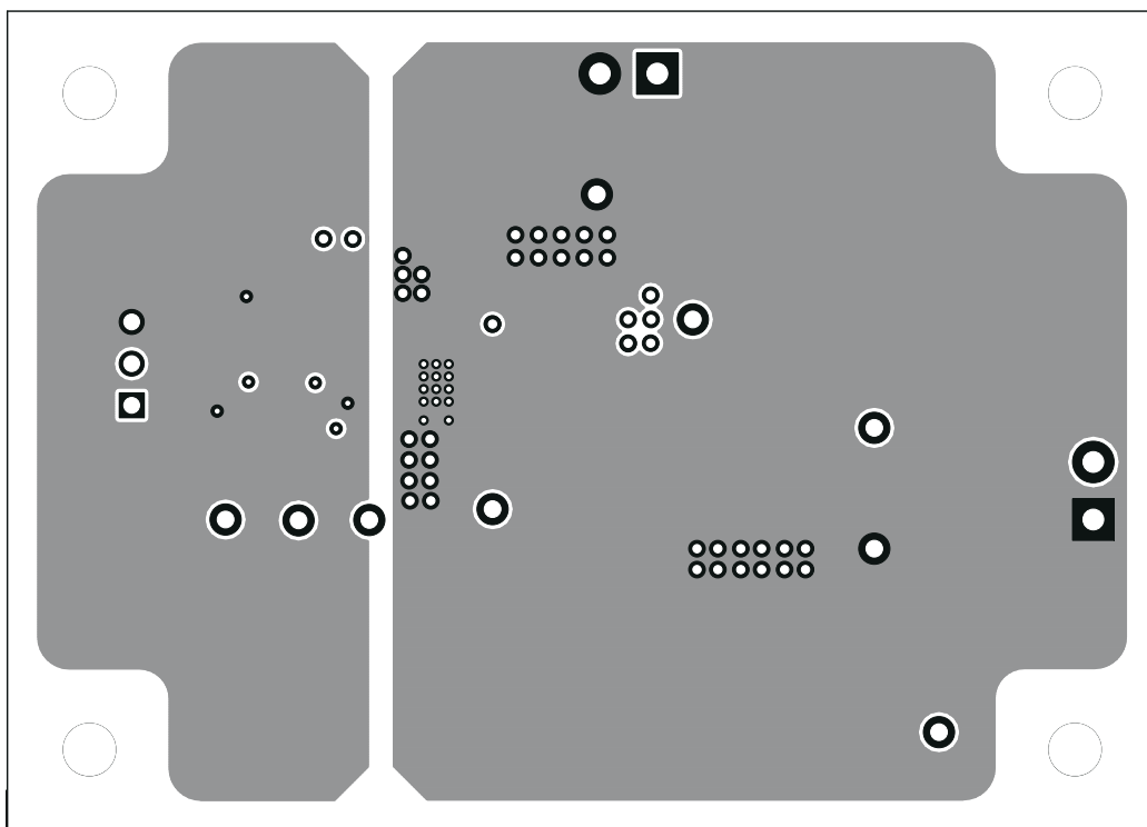
Figure 6-3. Internal Layer 1
