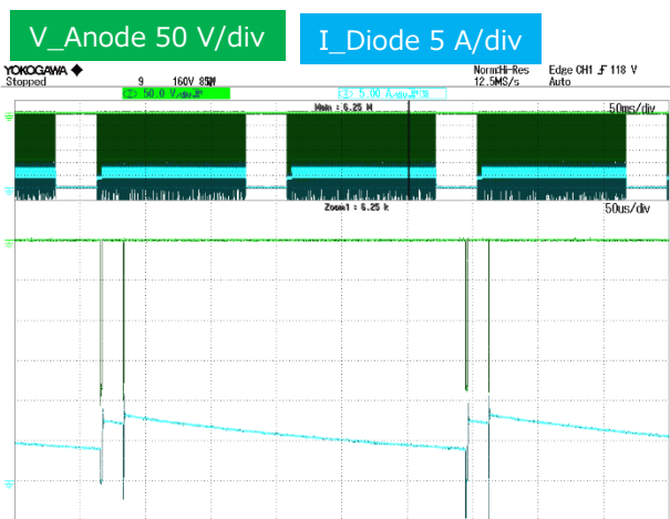
Figure 21. Output short V_{in\_dc} = 900\text{ V} Secondary side
