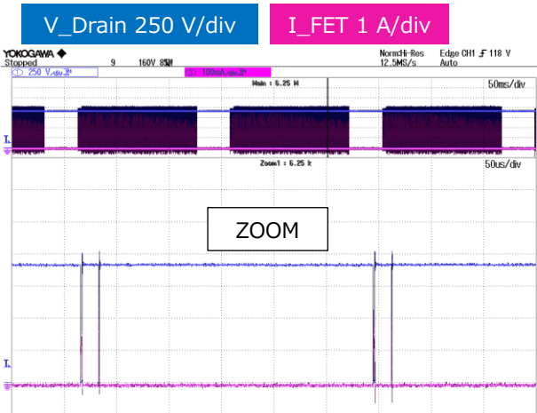
Figure 19. Output short V_{in\_dc} = 900\text{ V} Primary side
