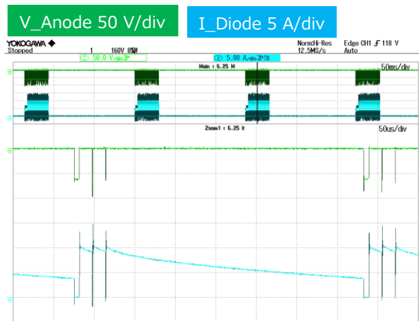
Figure 20. Output short V_{in\_dc} = 300\text{ V} Secondary side
