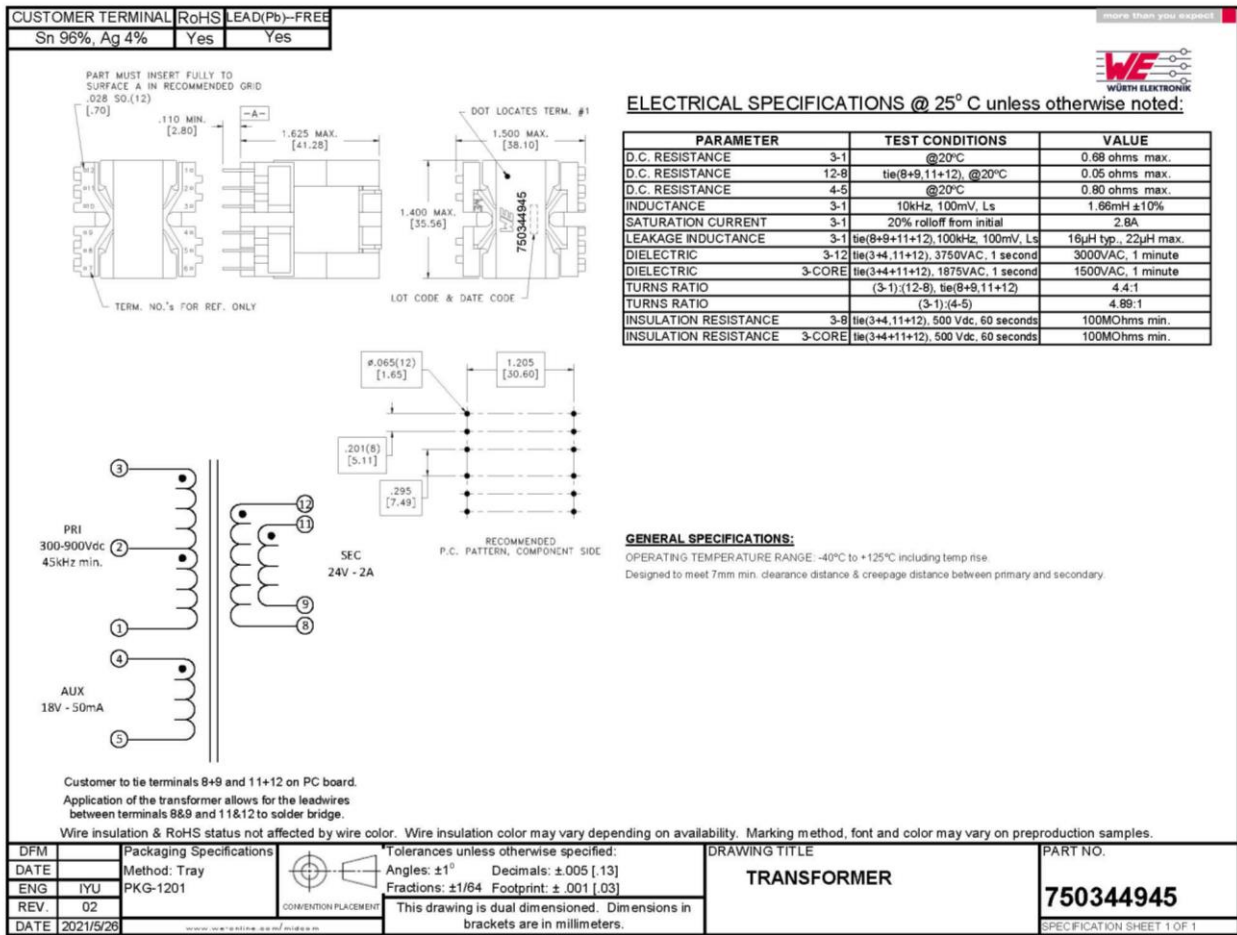
Figure 5. Transformer Specification
