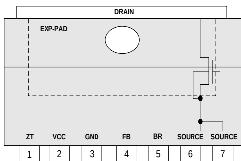
Figure 4. Pin Configuration
