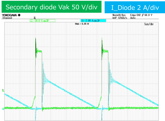
Figure 17. V_{in\_dc} = 900\text{ V} , I_o = 2.0\text{ A} Secondary Side
