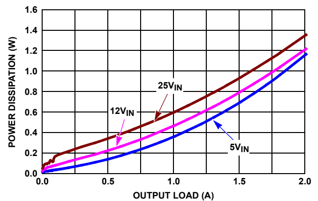
FIGURE 5. POWER DISSIPATION vs LOAD, 2.5\text{V}_{OUT}
