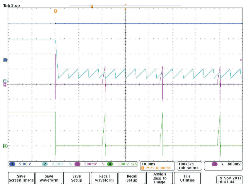
Figure 9-10. Over-Current Protection Waveform (Ch1: VIN, Ch2: EN/SS, Ch3: VOUT, Ch4: IOUT (10 A/div), VIN = 12 V, VOUT = 1.0 V, IOUT = 23 A)
