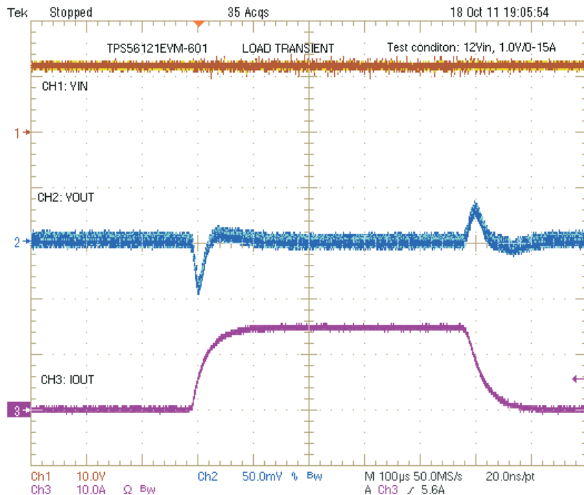
Figure 9-6. Load Transient (VIN = 12 V, VOUT = 1.0 V, IOUT = 0 A to 15 A)
