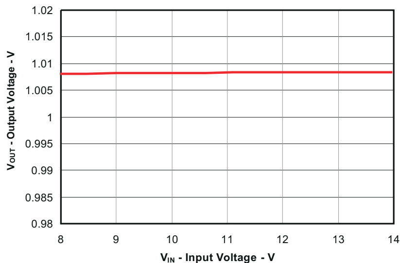
Figure 9-3. Line Regulation (V IN = 8 V to 14 V, V OUT = 1.0 V, I OUT = 15 A)
