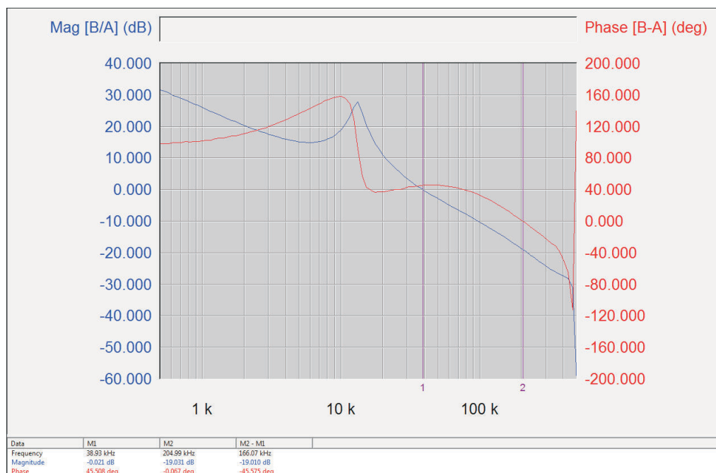
Figure 9-11. Loop Gain ( V_{IN} = 12\text{ V} , V_{OUT} = 1.0\text{ V} , I_{OUT} = 15\text{ A} , Bandwidth: 39 kHz, Phase Margin: 46°)
