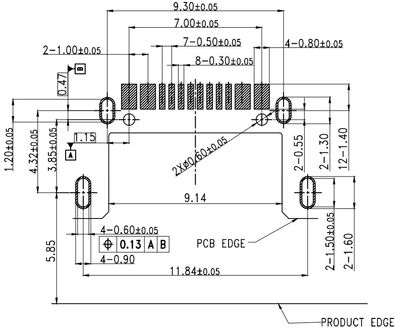
RECOMMENDED PCB LAYOUT (Tolerance=±0.05)
