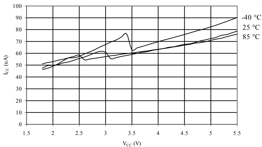
Figure 30-43. AREF External Reference Current vs. V_{CC}
