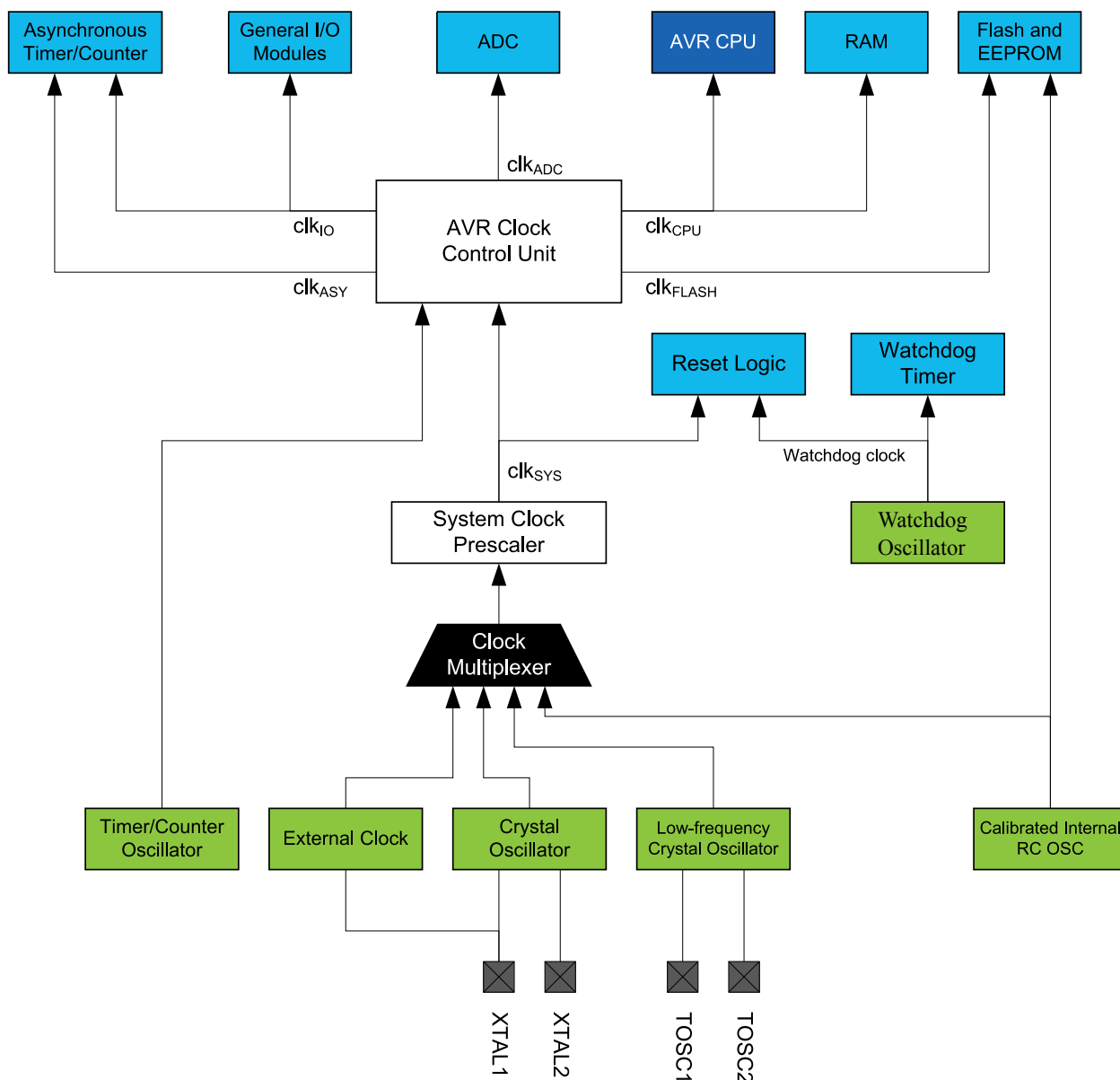
Figure 10-1. Clock Distribution
