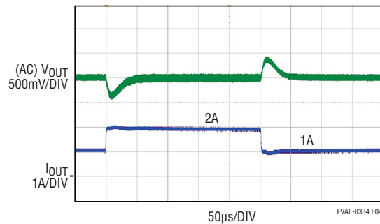
Figure 4. EVAL-LT8334-AZ V_{OUT} Transient Response with V_{IN} = 12V , V_{OUT} = 12V , I_{OUT} = 1A to 2A (JP1 = PULSE SKIP)
