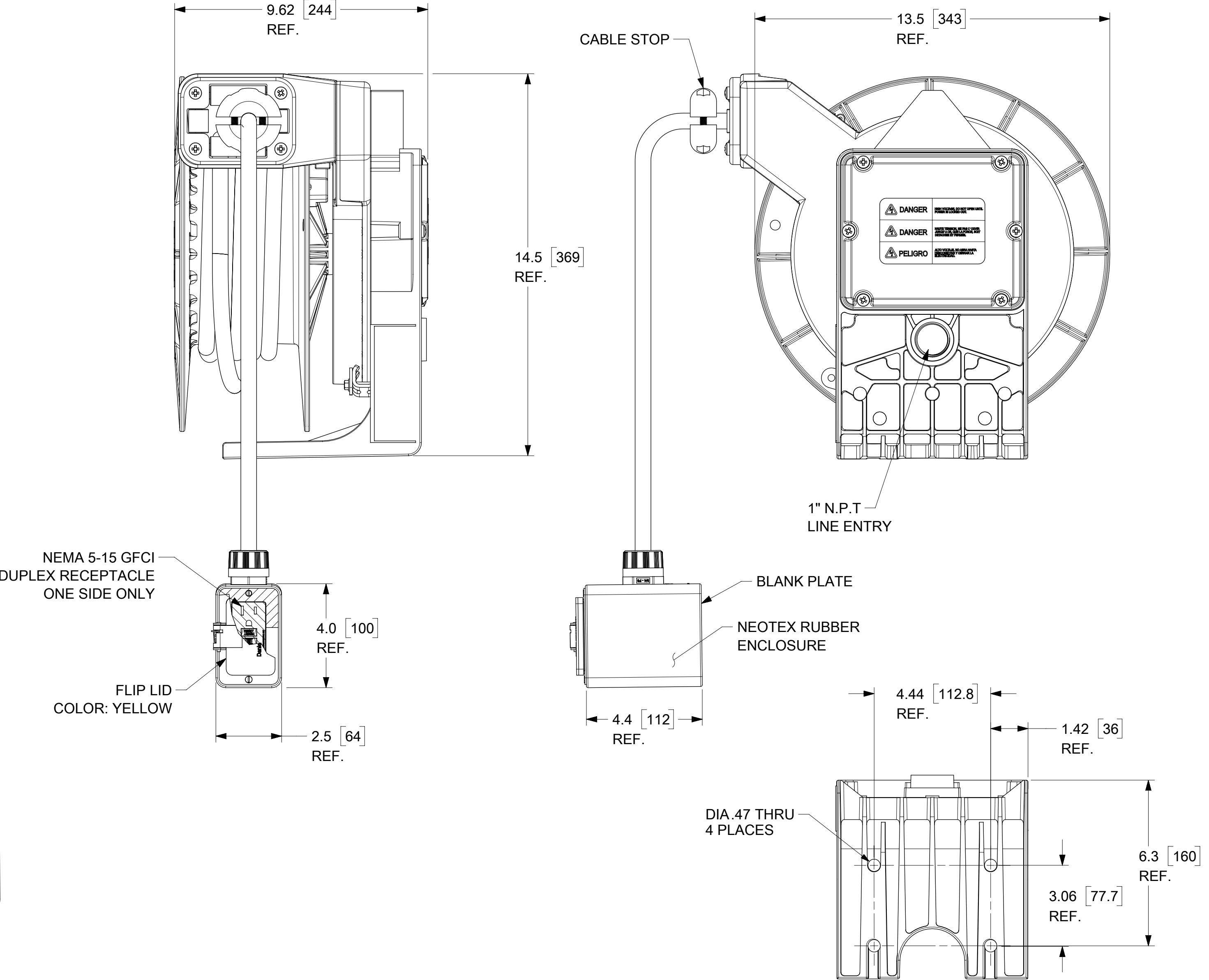
BOTTOM VIEW
